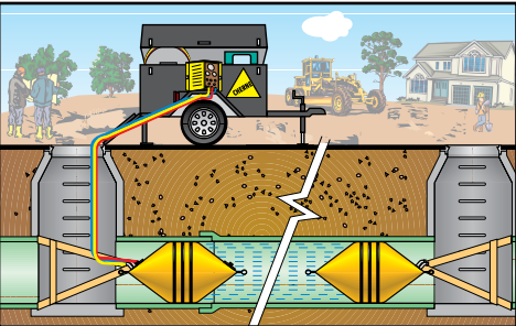
Sewer air test
