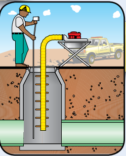
Blow-in ventilator
