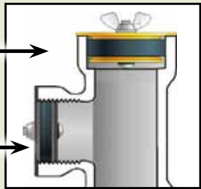
Hub-Fit Gripper® plug
