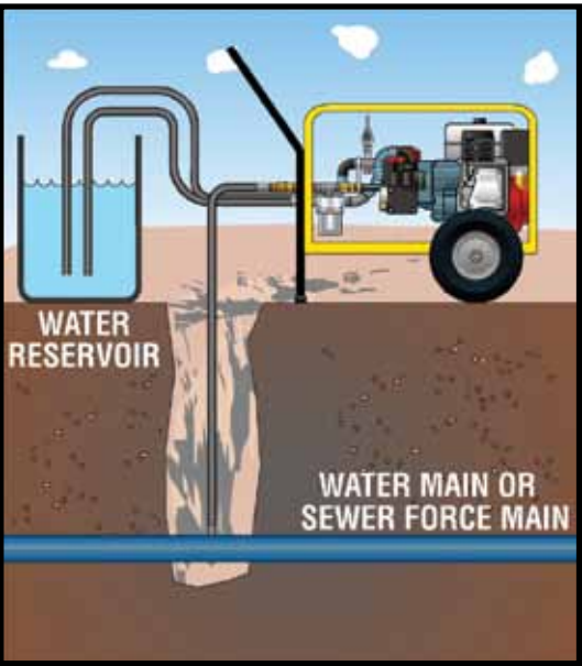
Suction Feed
