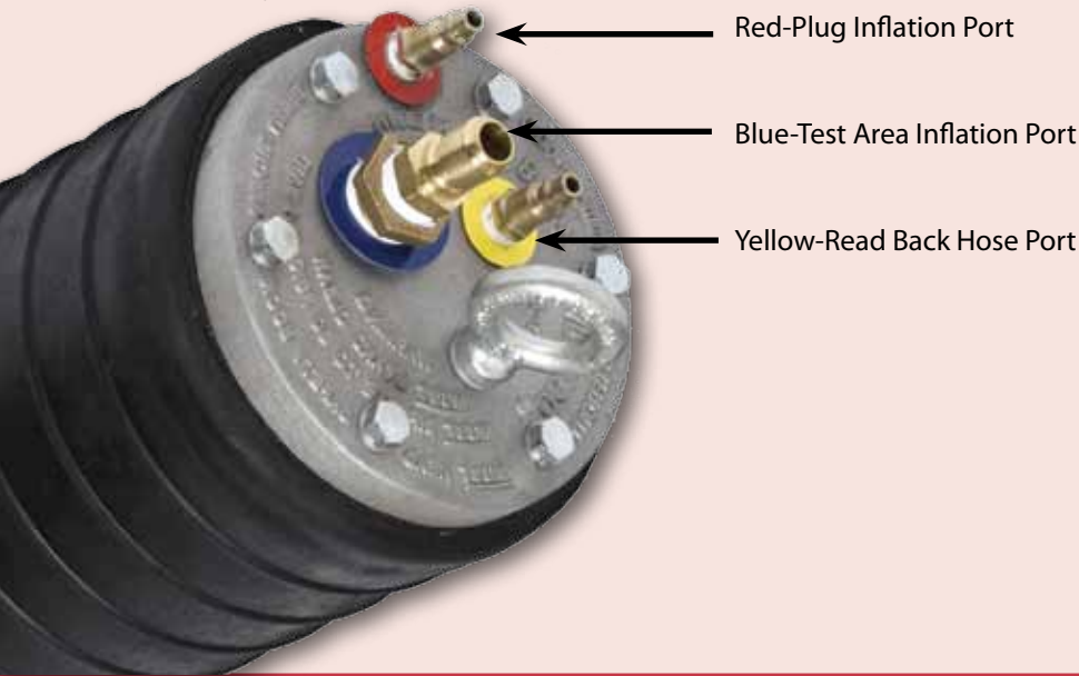
Front Plug
