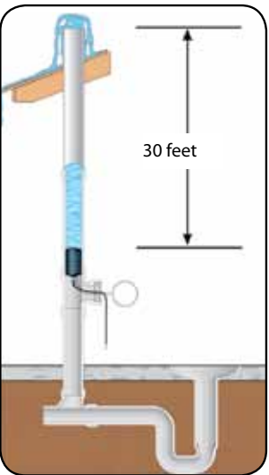
In the example above, the answer is: 30 feet of pipe above the plug = 30 feet of head
