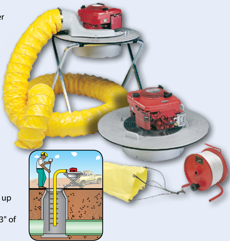
Blow-in ventilator
