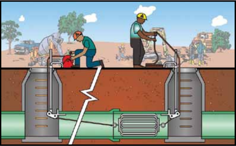
Deflection Test
